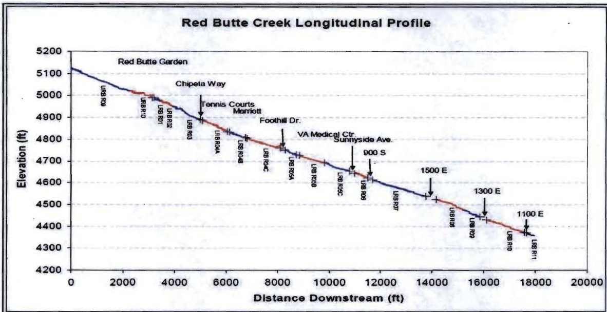
Figure 2. Elevation Profile of Red Butte Creek. Diagram from SLC Riparian Corridor Restoration Study Final Red Butte Creek Management Plan.
